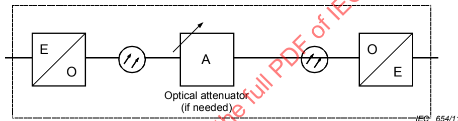
Figure 10 – Device under test for measuring CSO of optical transmitters
