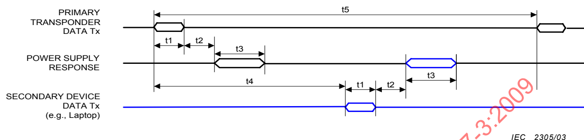
Figure 5 – PSTIB data and timing diagram
