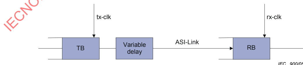
Figure F.1 – Abstract ASI transmission model
