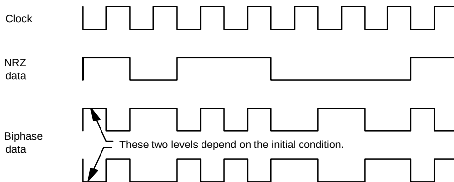
Figure A.6a – Biphase Mark coding scheme
