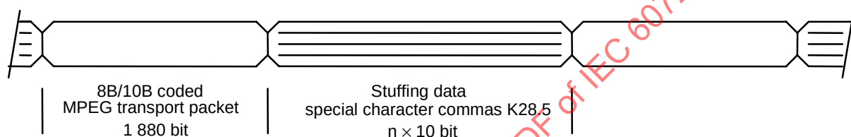
Figure B.7 – Transmission format with data packets (example for 188 bytes)
