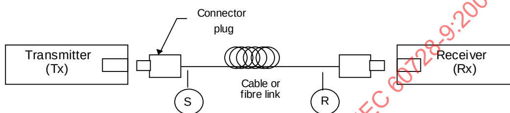
Figure B.3 – Serial link Layer-0 reference points
