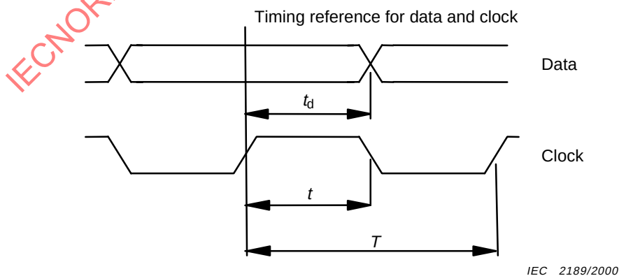
Figure 9 – Clock to data timing (at source)
