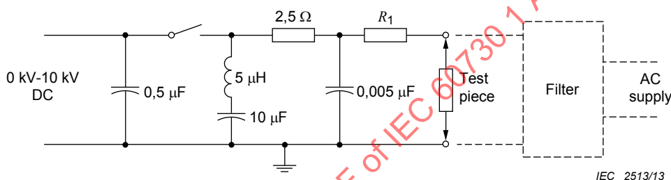
Figure H.4 – Schematic of a ring wave generator 0,5 μs / 100 kHz
