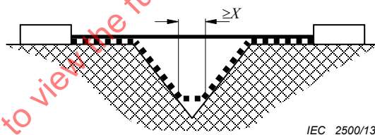
Figure B.2 – Encoche large
