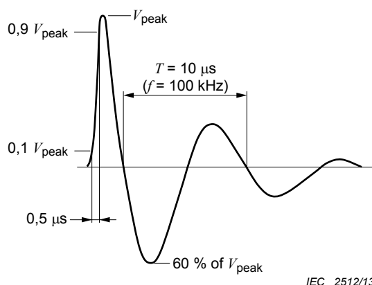
Figure H.3 – Ring wave characteristics (open-circuit voltage)
