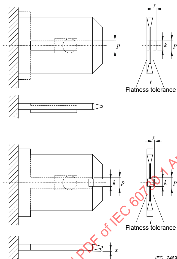
Figure 15 – Tabs for non-reversible connectors
