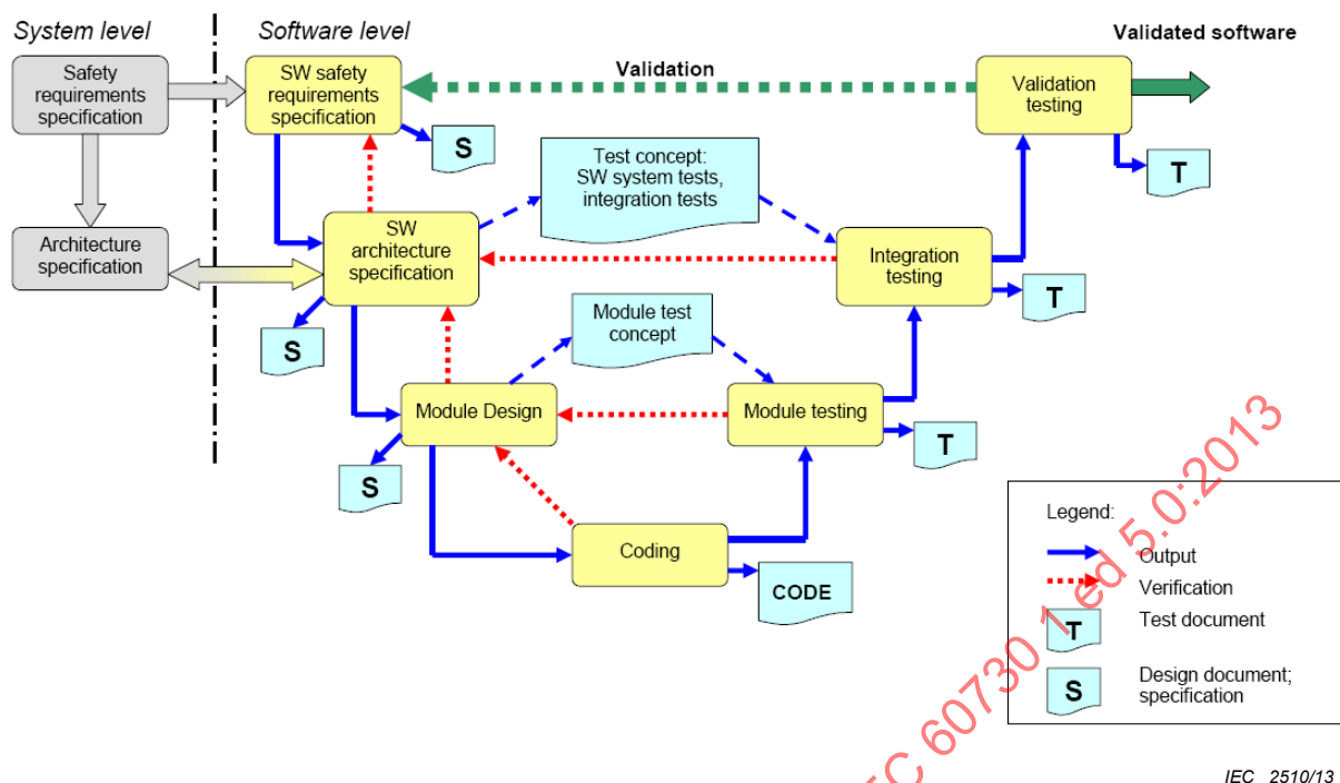
Figure H.1 – V-Model for the software life cycle
