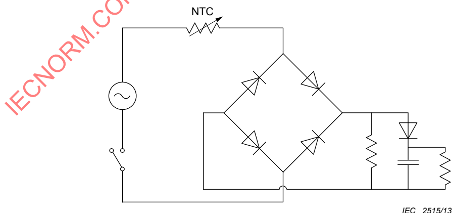
Figure J.1 – Test circuit for inrush-current limiting thermistor endurance test
