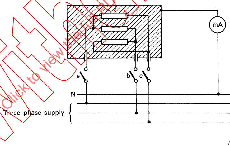
Figure 28 – Diagram for leakage current measurement at operating temperature for three-phase connection of controls other than those of class II
