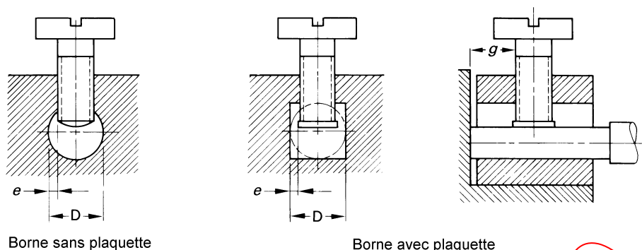
Borne sans plaquette
