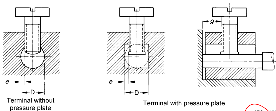
Figure 11 – Pillar terminals
