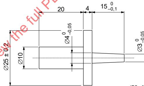
Figure 1 – Test pin
