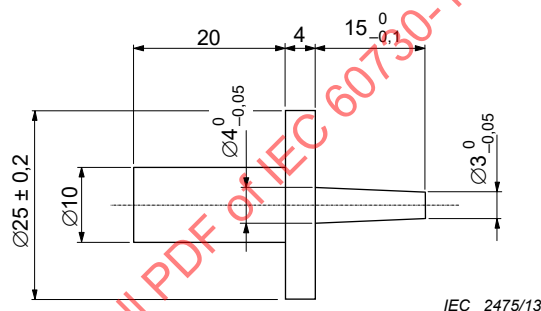
Figure 1 – Test pin
