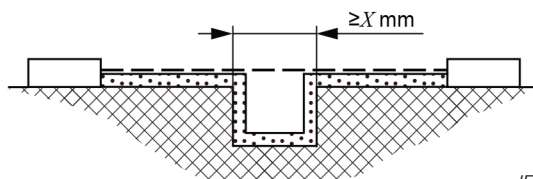
Figure B.1 – Narrow groove
