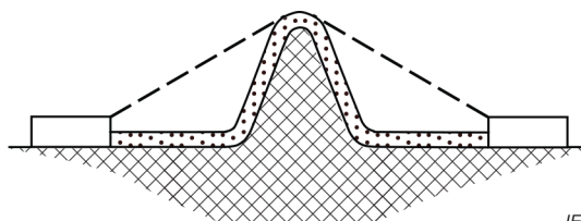
Figure B.3 – V-shaped groove
