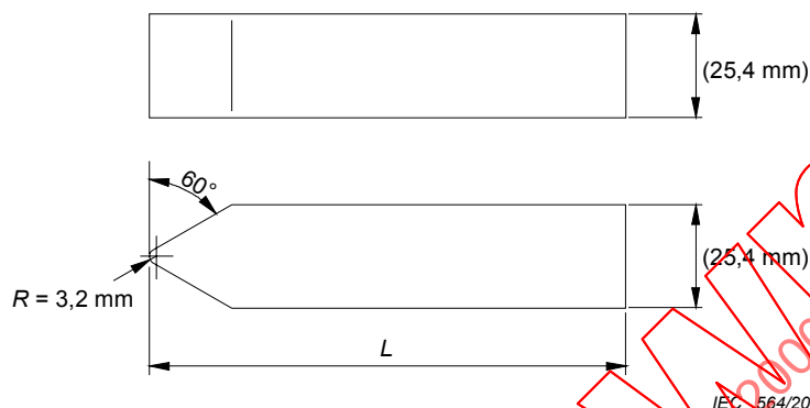
Figure 11.4.13.102 – Outil de frappe
