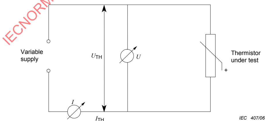
Figure 6 – Dissipation factor test circuit
