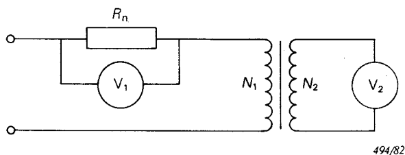
FIG. 2. — Measurements at low and medium field strengths.
