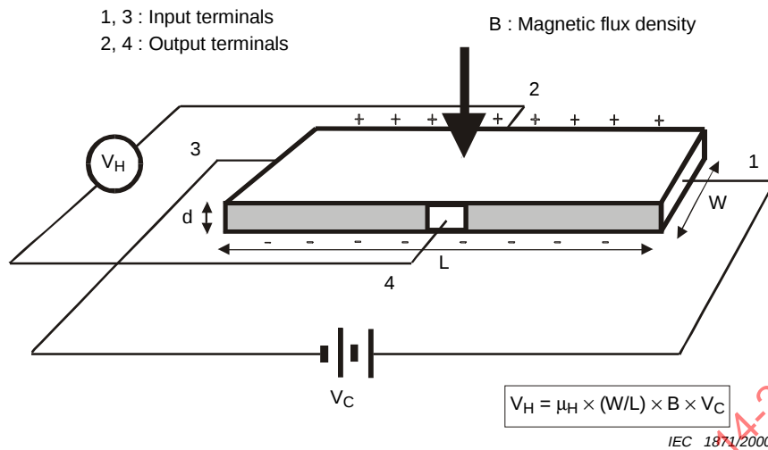
Figure 1 – The principles of Hall element
