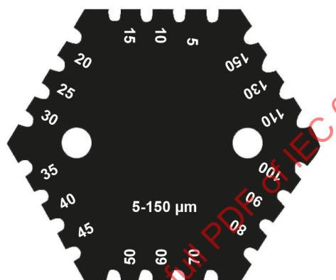
Figure B.1 – Example of a measuring gauge for a layer of thermal compound paste of a thickness between 5 µm and 150 µm
