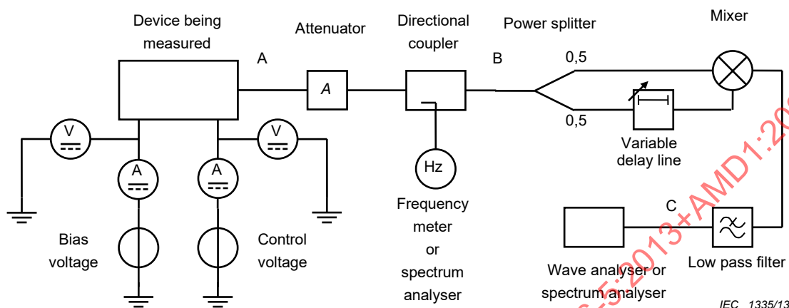
Figure 3 – Circuit diagram for the measurement of the phase noise \mathcal{S}(f) (method 2)
