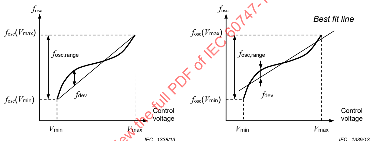
Figure 6 – Tuning linearity
