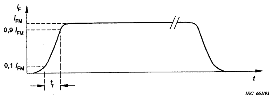
Figure 42a - Current waveform
