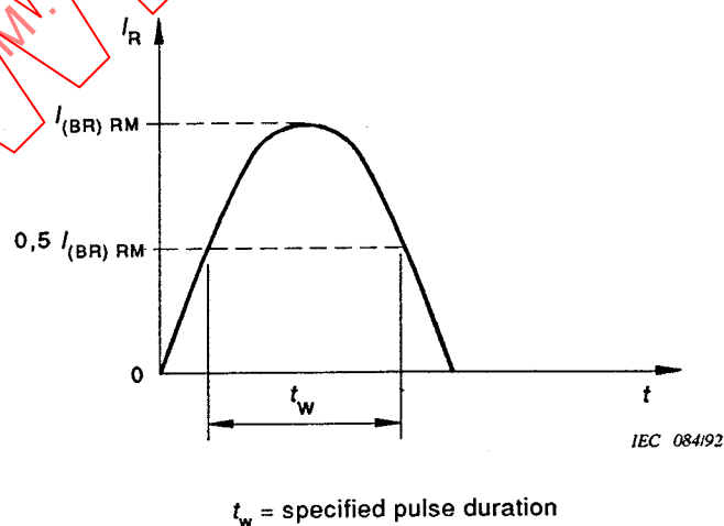
Figure 46 - Reverse current waveform
