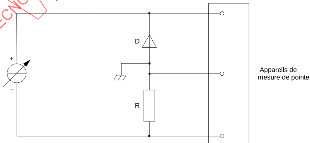
Figure 14 – Schéma
