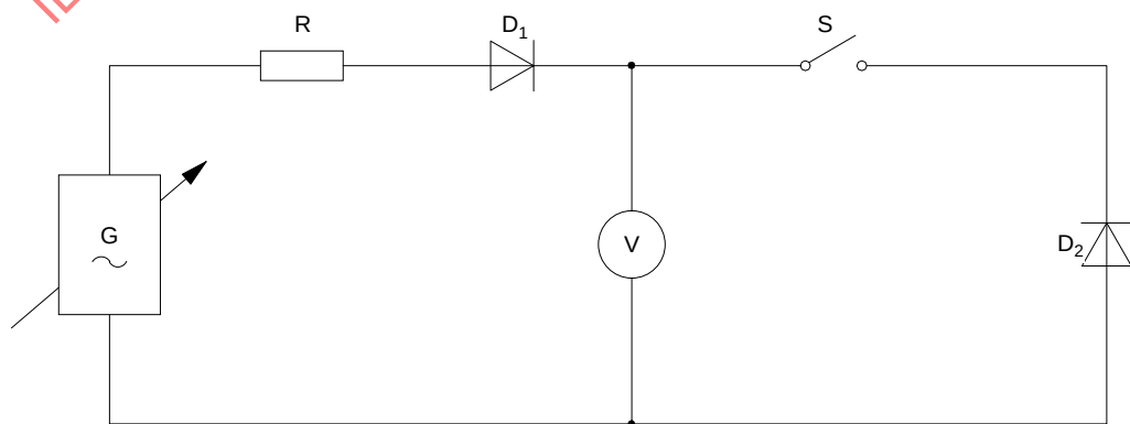
Figure 28 – Circuit diagram
