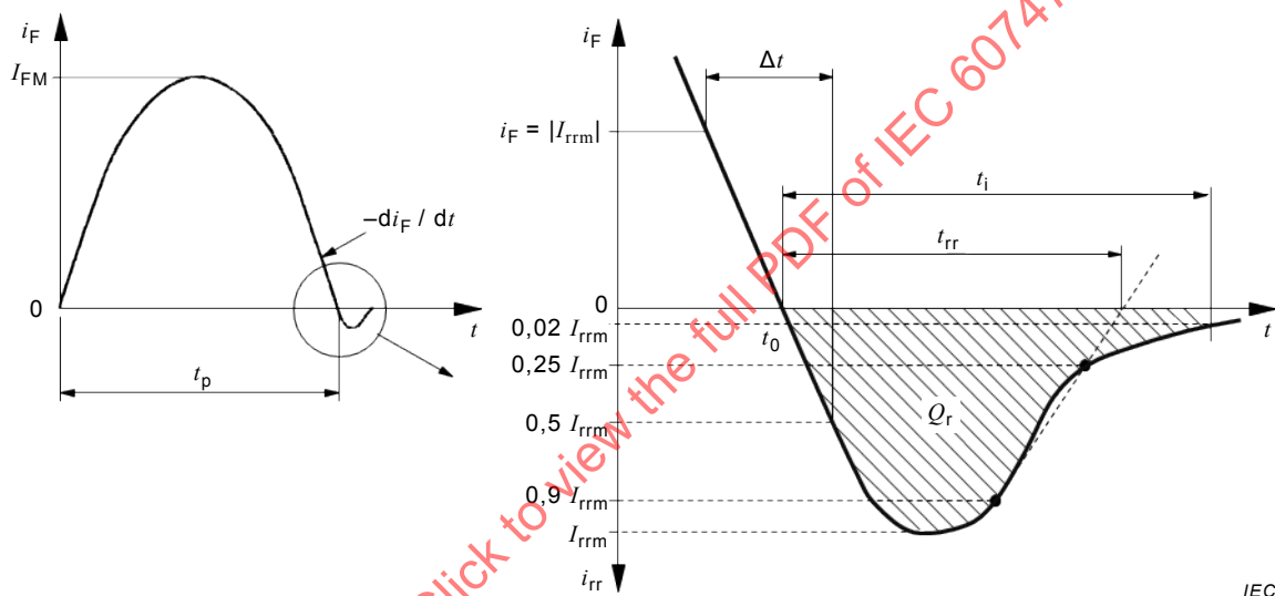
Figure 16 – Current waveform through the diode D during recovered charge measurement, half sinusoidal wave method
