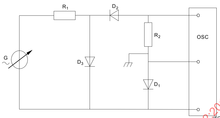
Figure 14 – Circuit diagram for peak reverse current measurement
