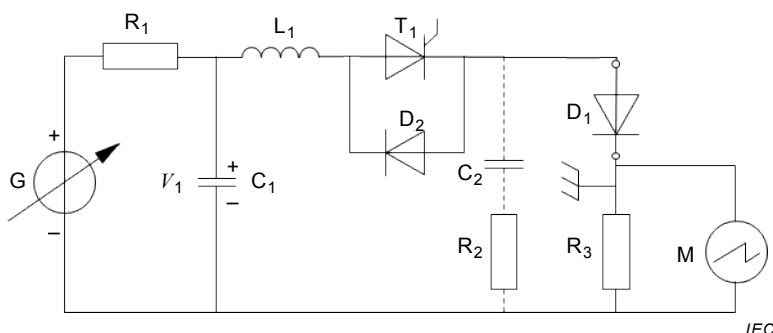
Figure 15 – Circuit diagram for recovered charge measurement, half sinusoidal wave method
