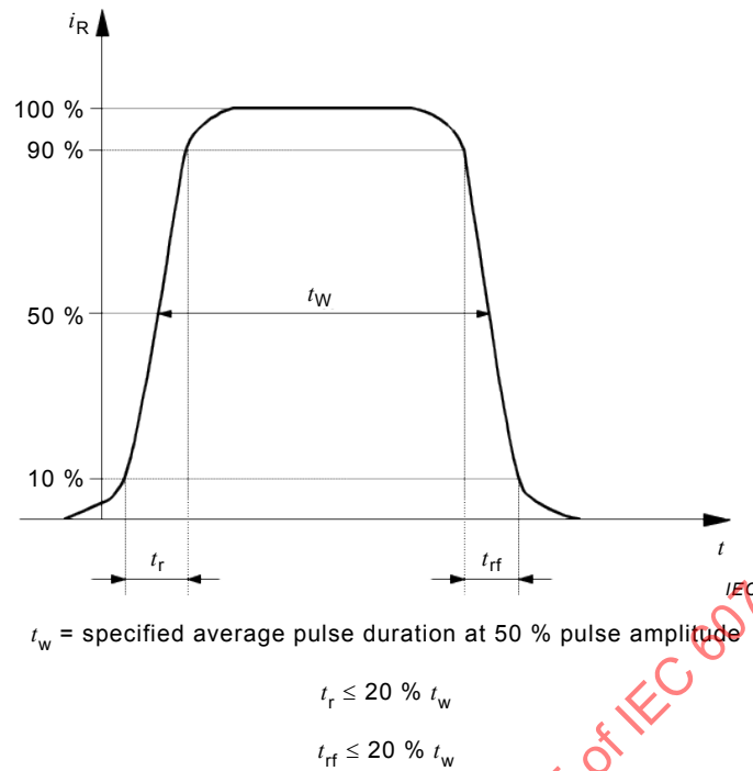
Figure 30 – Rectangular reverse current waveform
