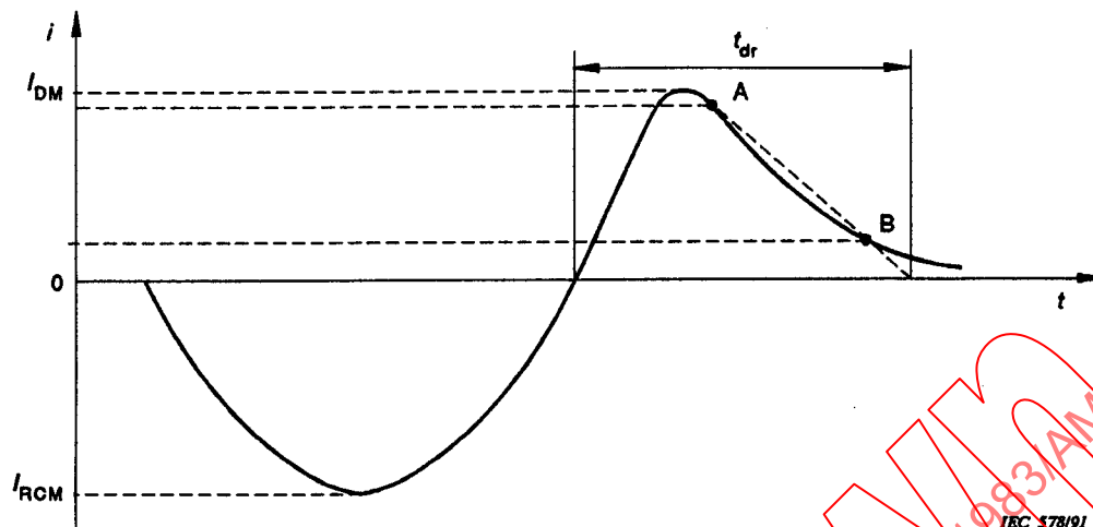
Figure 6 – Current waveforms
