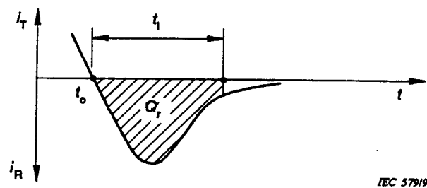
Figure 71 – Recovered charge
