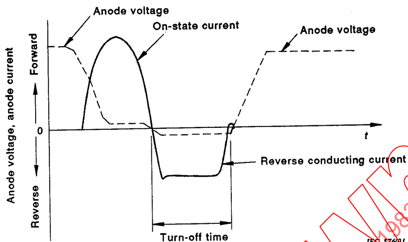
Figure 70 – Circuit commutated turn-off time
