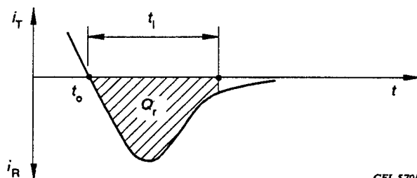
Figure 71 – Charge recouvrée
