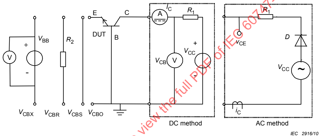
Figure 7 – Circuit for testing the collector-base voltage V_{CBO} , V_{CBS} , V_{CBR} , V_{CBX}
