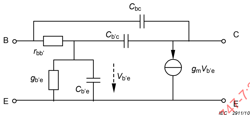
Figure 2 – Modified hybrid \pi equivalent circuit
