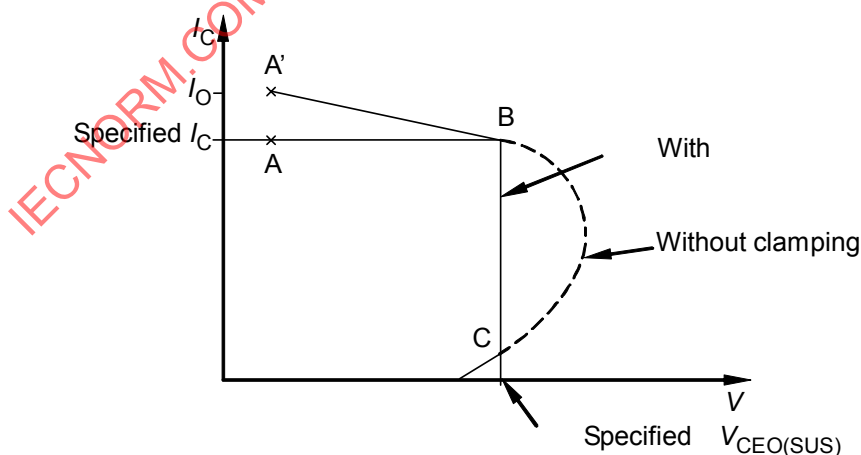
Figure 16 – I_{\text{C}} versus V_{\text{CE}} characteristic
