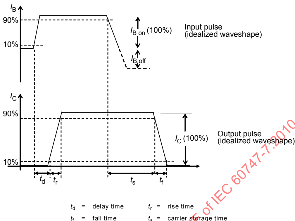
Figure 37 – Switching times
