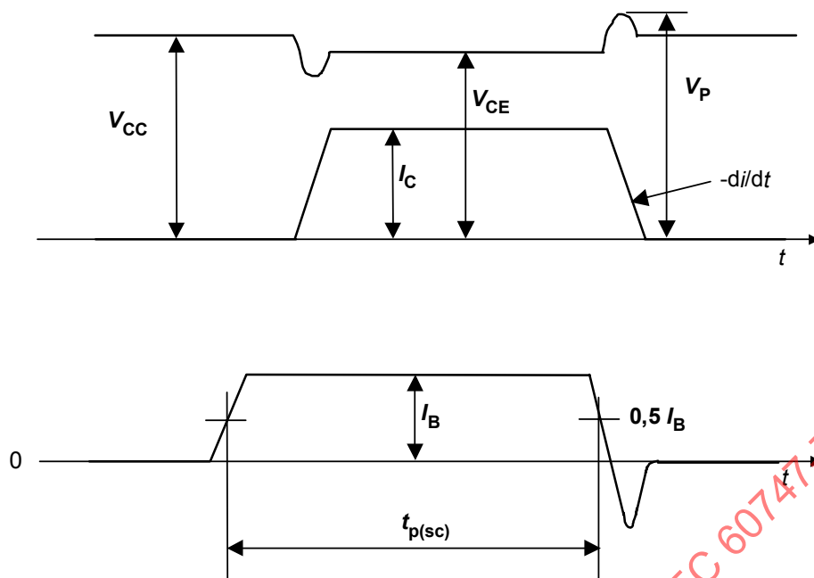
Figure 13 – Waveforms of base current I_B , collector current I_C and voltage V_{CE} during load short circuit condition SCSOA
