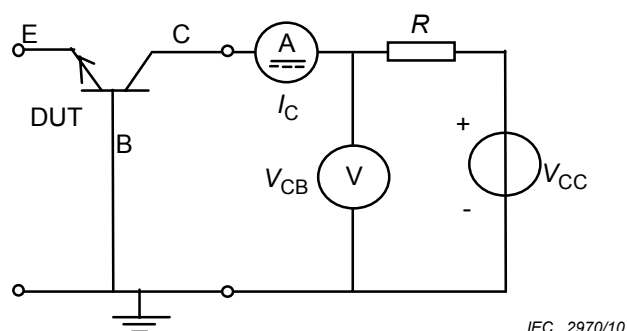
Figure 57a – Circuit for high temperature blocking (Method 1)
