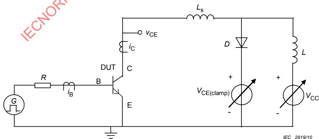
Figure 10 – Test circuit of reverse bias safe operating area (RBSOA)
