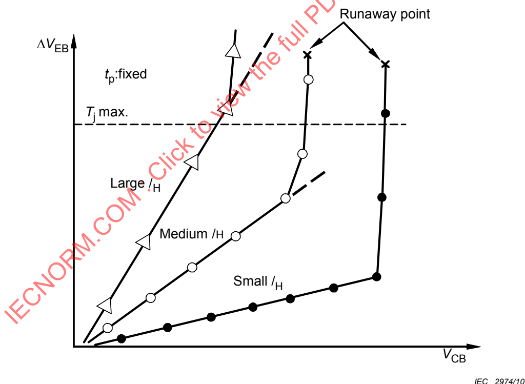
Figure A.1 – Typical \Delta V_{EB} versus collector-base ( V_{CB} ) characteristics
