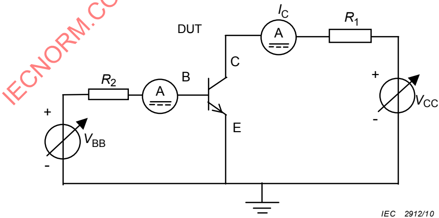
Figure 3 – Test circuit for collector current
