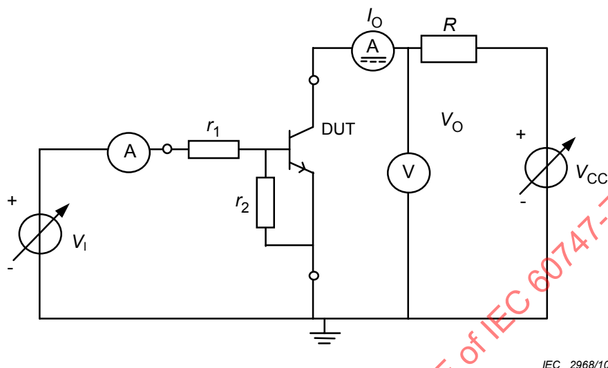
Figure 55 – Circuit diagram for measuring the on-state output voltage V_{O(on)}
