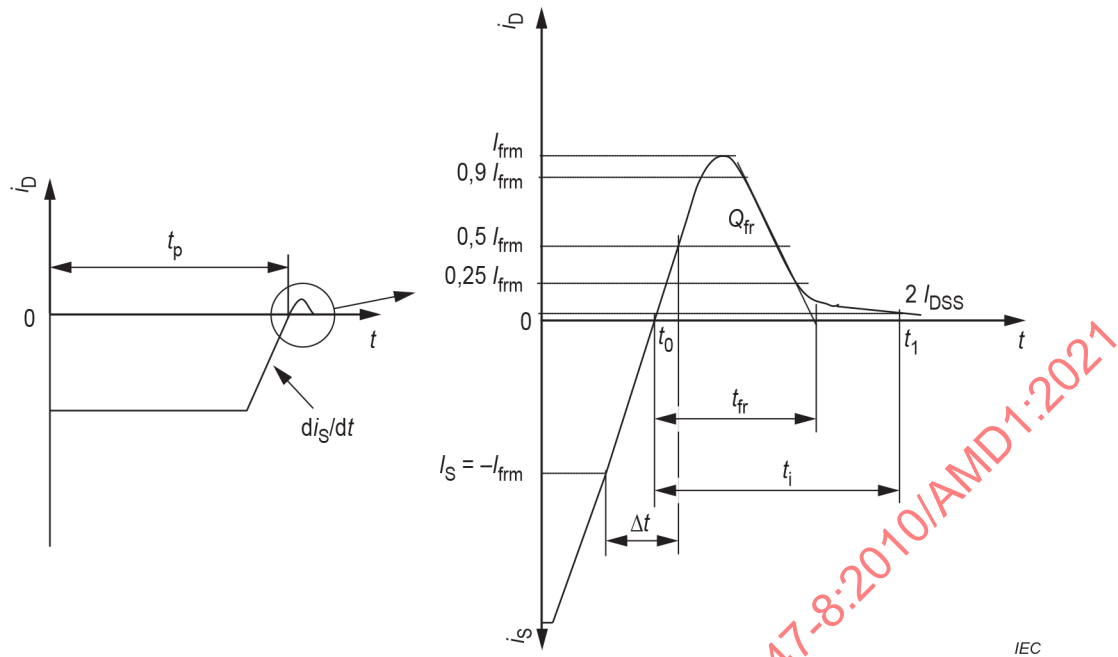
Figure 34 – Current waveform through MOSFET (Method 1)
