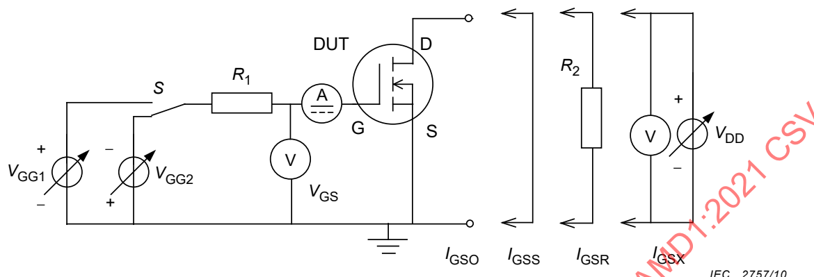
Figure 22 – Circuit diagram for measuring of gate cut-off current or gate leakage current
