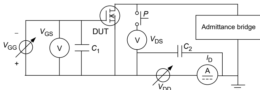
Figure 38 – Basic circuit for the measurement of the output conductance g_{oss} (method 1: null method)
