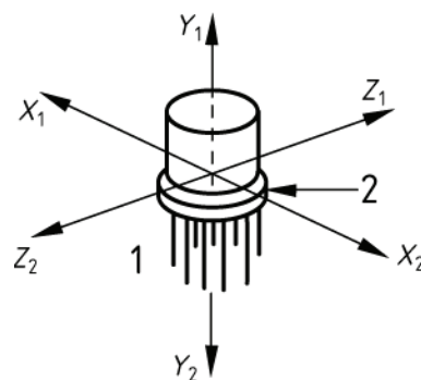
Figure 1e – Cylindrical package
