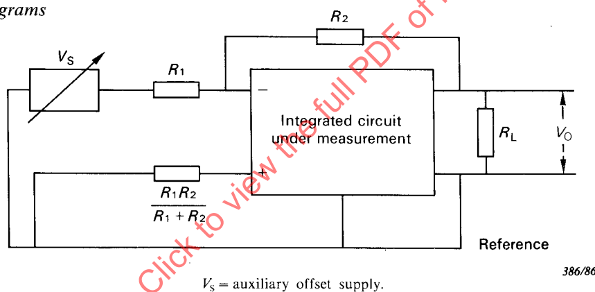
FIG. 14. — Differential inputs.
