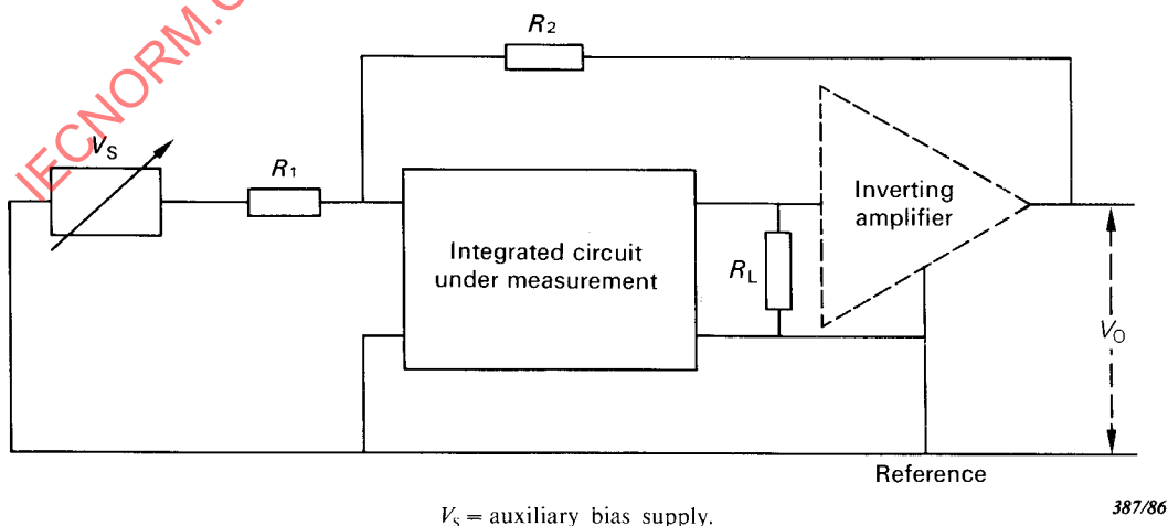
FIG. 15. — Single-ended input.
