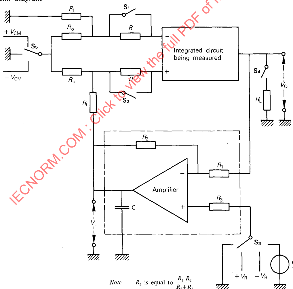
FIG. 31. — Measurement circuit.
