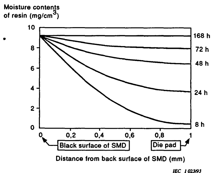
Figure 5 – Process of moisture diffusion at 85 °C, 85 % RH
