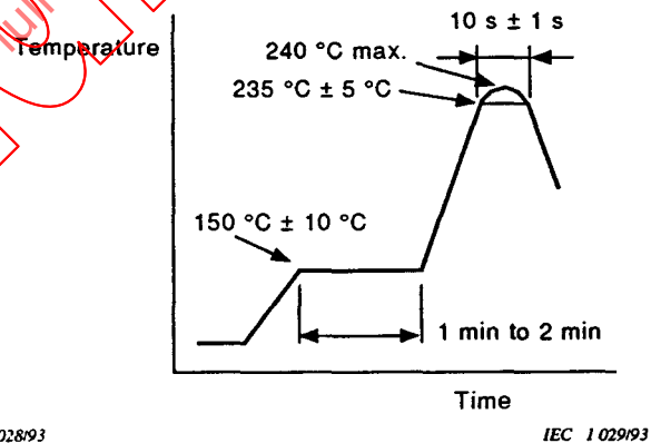
Figure 11 – Temperature profile of infrared reflow soldering
