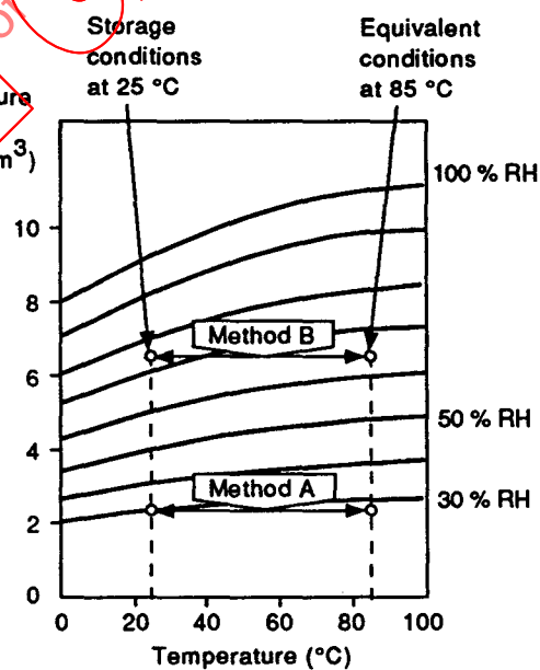
Figure 8 – Temperature dependence of saturated moisture content of resin
