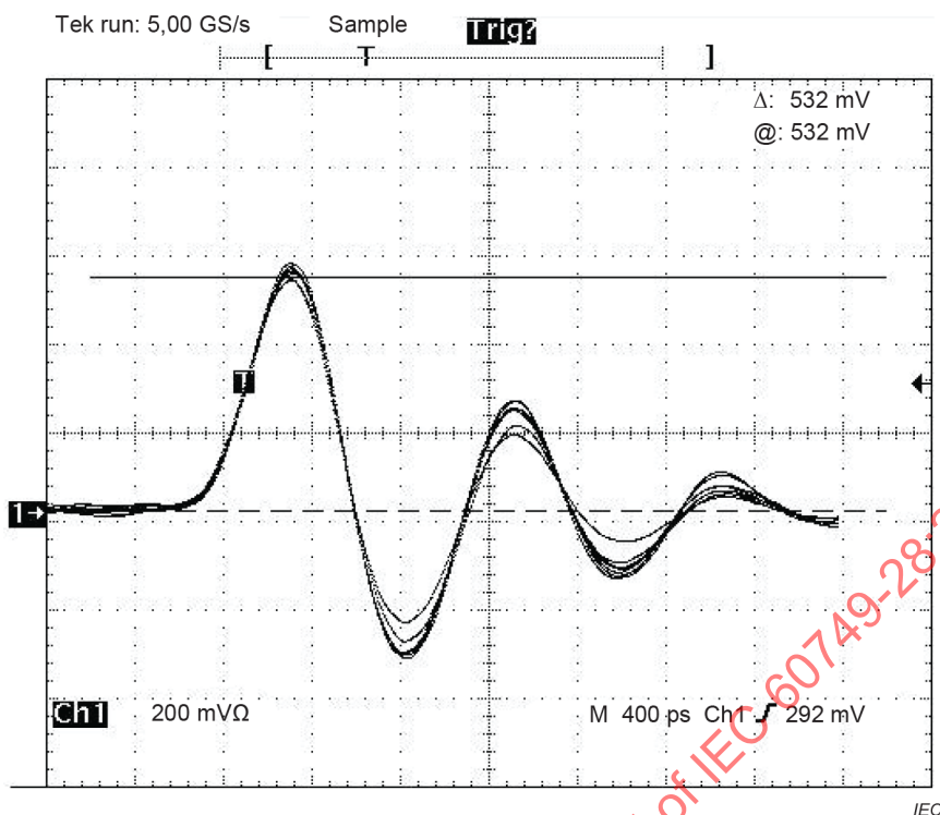
Figure F.1 – 1 GHz TC 500, small verification module
