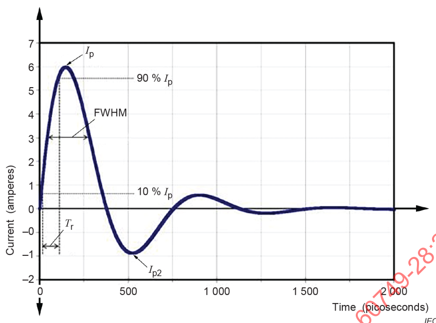
Figure 2 – CDM characteristic waveform and parameters
