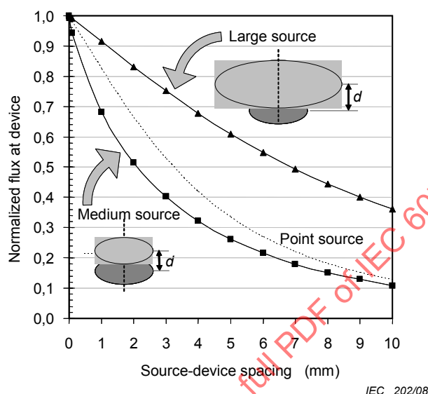
Figure 1 – Effect of source-device spacing on normalized flux at device
