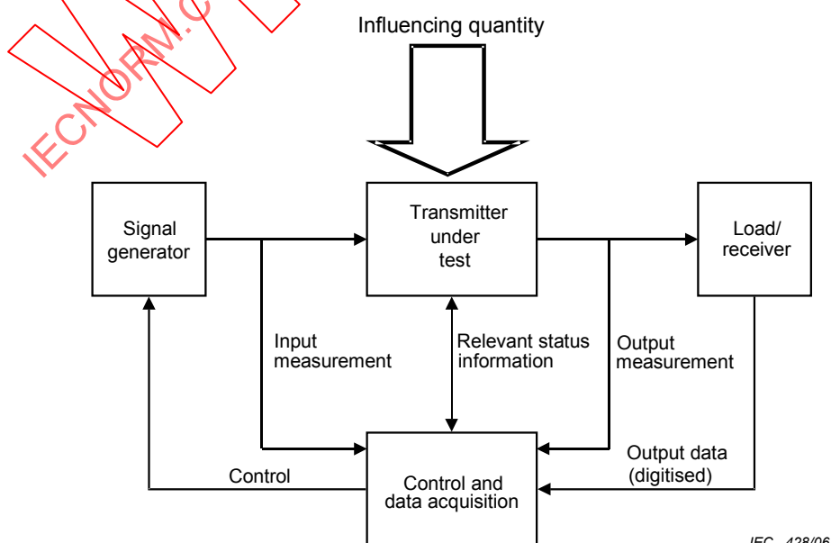
Figure 2– Basic test set-up
