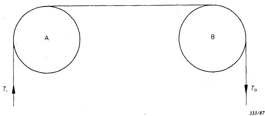
FIG. 7. — Constant strain proof test apparatus.
