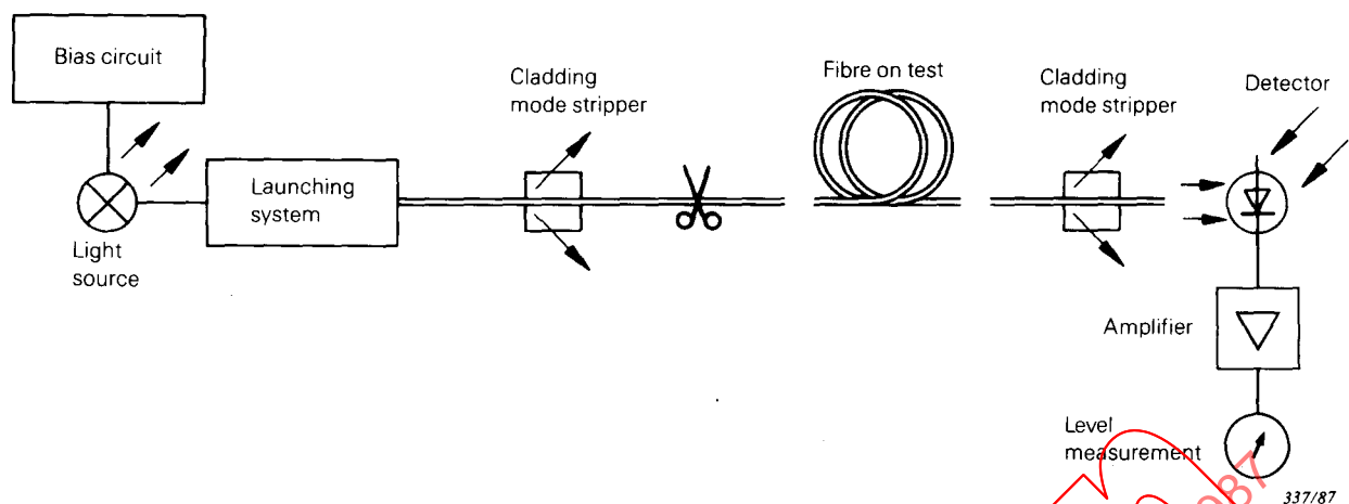
FIG. 11. — Arrangement of test equipment to make loss measurement at one specified wavelength.
