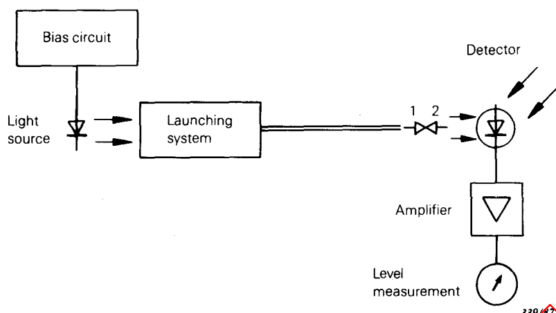
FIG. 13. — Calibration of insertion loss measuring set.
