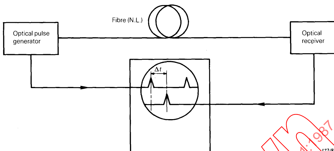
FIG. 3a. — Time measurement of the transmitted pulse.
