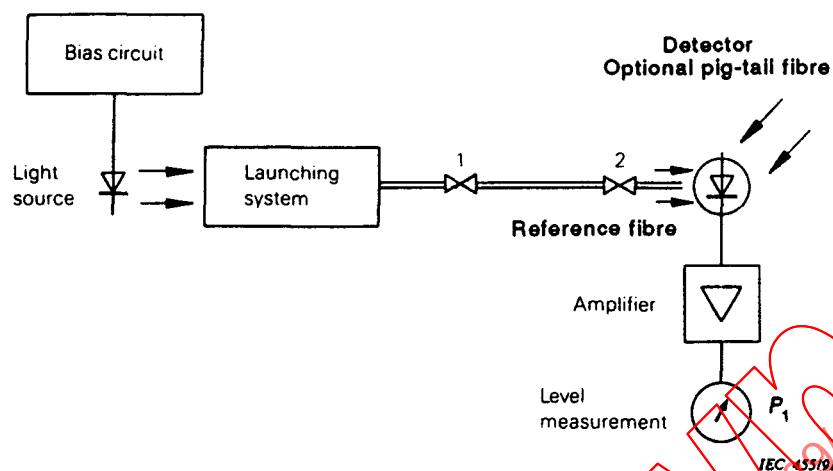
Figure 14 - Calibration of insertion loss measuring set
