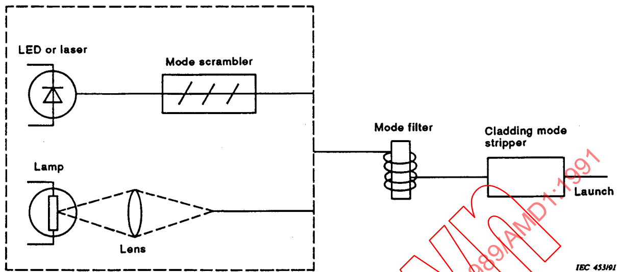
Figure 11A - Arrangement of test equipment to make loss measurement at one specified wavelength
