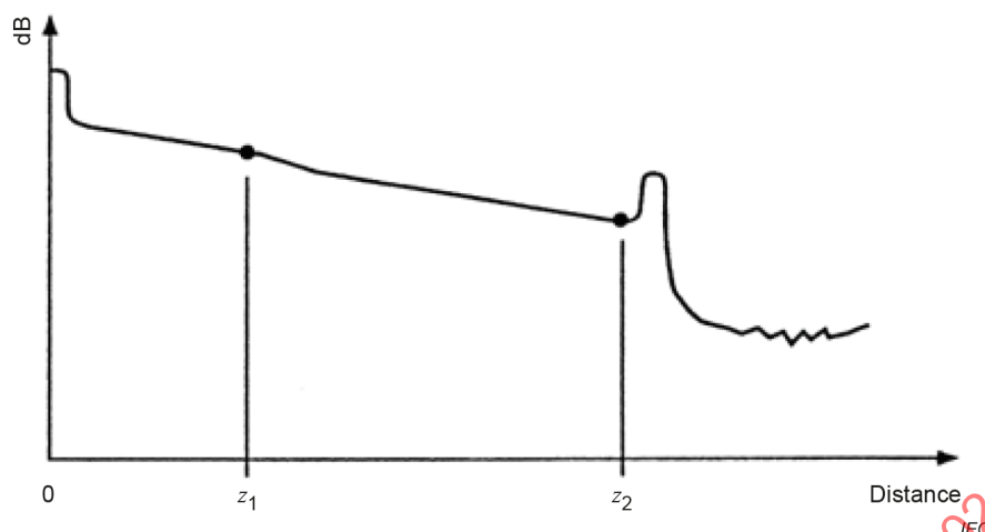
Figure B.2 – Schematic OTDR trace of a specimen sample ( z_1 to z_2 ) with a section (e.g. dead-zone fibre) of unknown length, z_1 , preceding it and without a reflection pulse from the fibre joint point (two-point technique (B.4.3.1))
