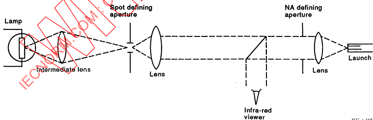
Figure 2 – Limited phase space launch optics
