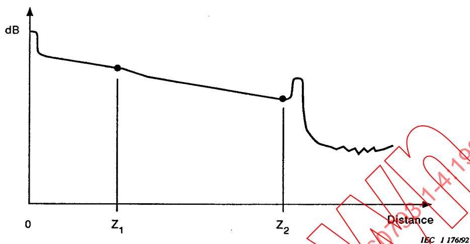
Figure 10 – Schematic OTDR trace of a test sample ( z_1 to z_2 ) with a section (e.g., dead-zone fibre) of unknown length z_1 , preceding it and without a reflection pulse from the fibre joint point (two-point method A)
