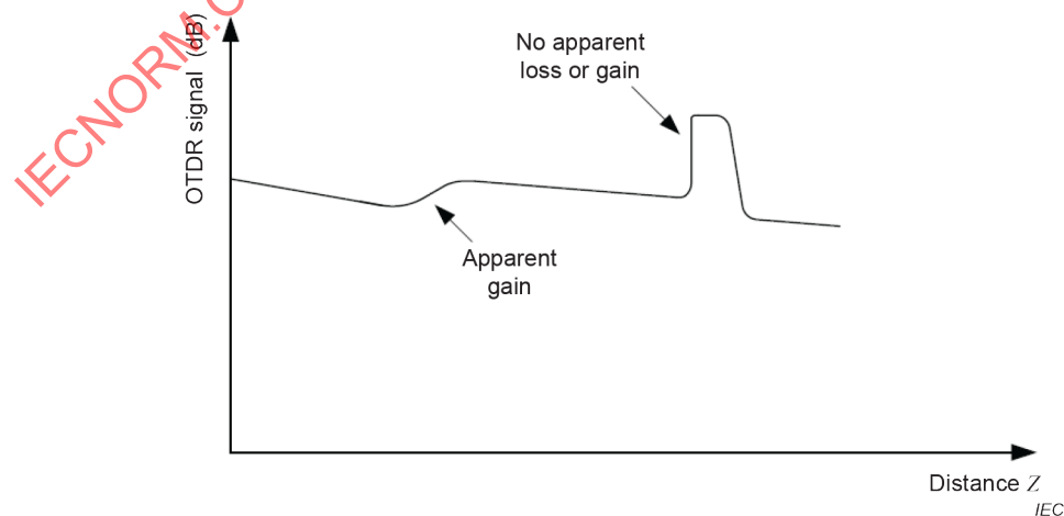
Figure C.5 – Schematic of an expanded OTDR trace showing two point discontinuities, one with apparent gain, and another with no apparent loss or gain
