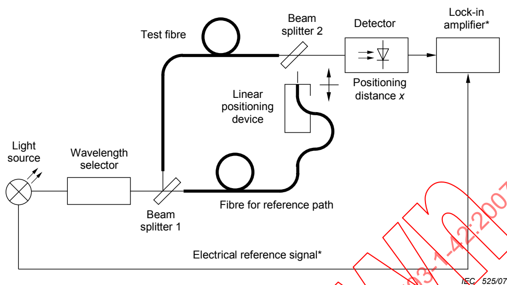
Figure D.1 – Fibre chromatic dispersion test set – Interferometry by fibre reference path
