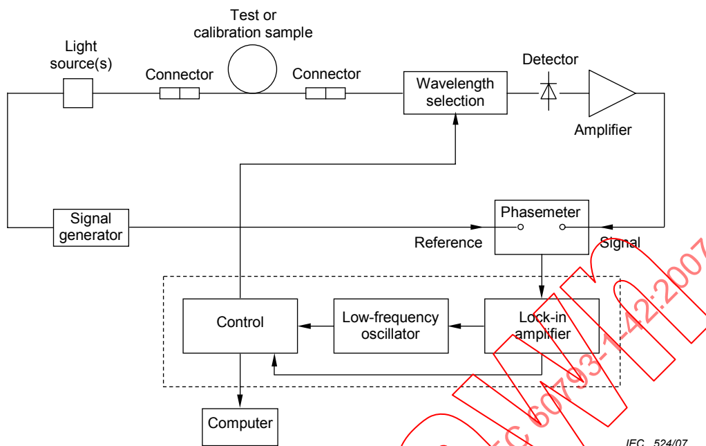
Figure C.4 – Chromatic dispersion measurement set, differential phase by double demodulation
