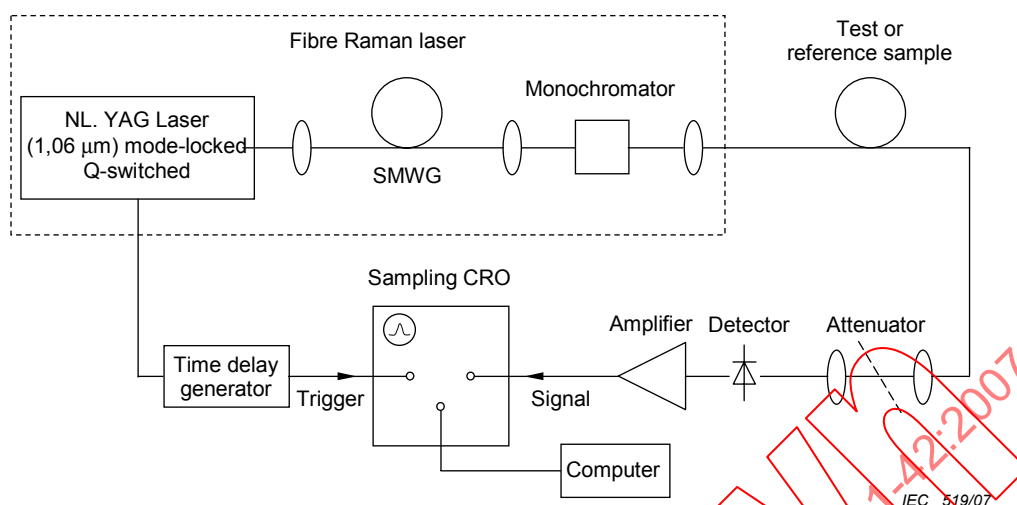
Figure B.1 – Block diagram, fibre Raman laser system
