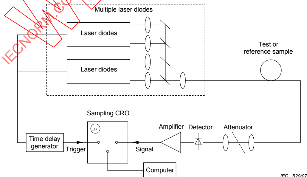
Figure B.2 – Block diagram, multiple laser diode system
