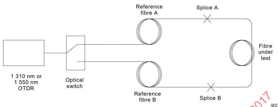
Figure D.1 – Optical switch arrangement
