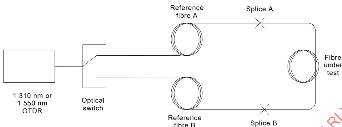
Figure D.1 – Optical switch arrangement
