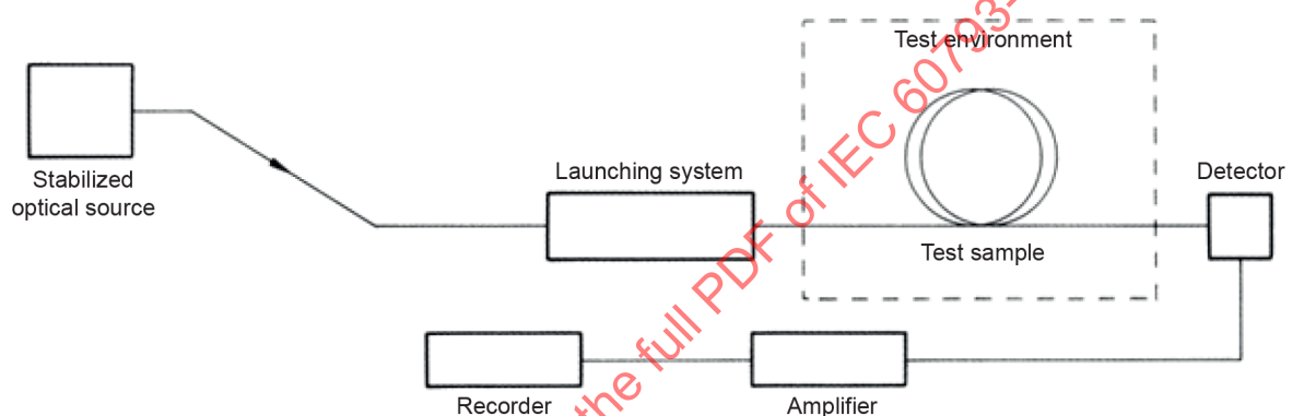
Figure A.2 – Measurement of change in attenuation using stabilized source
