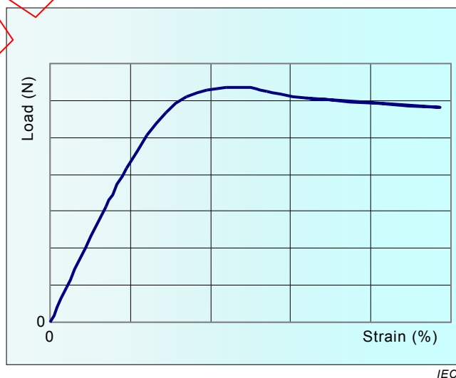
Figure 1 – Tensile load versus elongation for a plastic optical fibre
