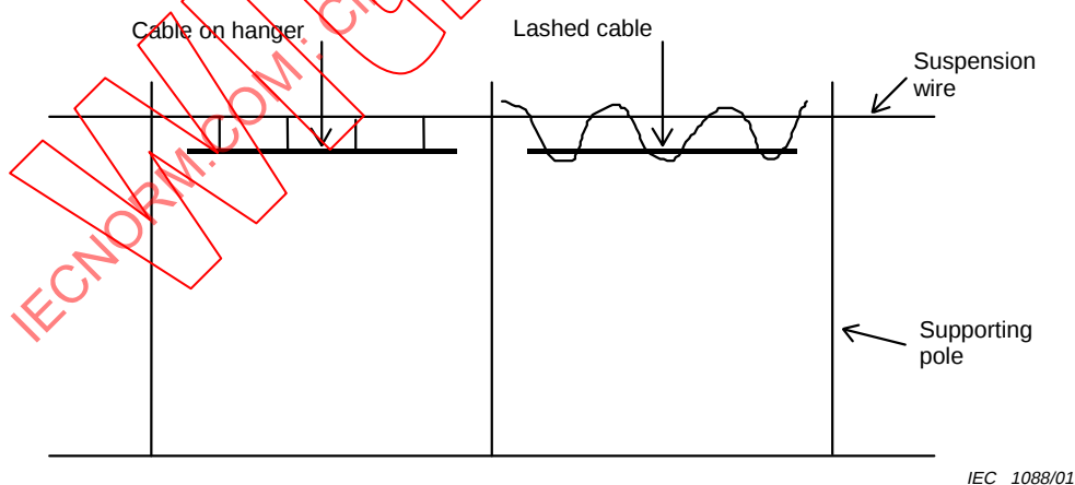
Figure A.3 – Aerial cable installation
