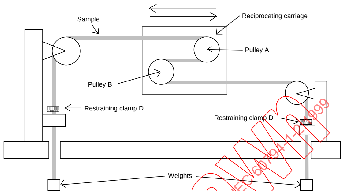
Figure 13 – Flexing apparatus
