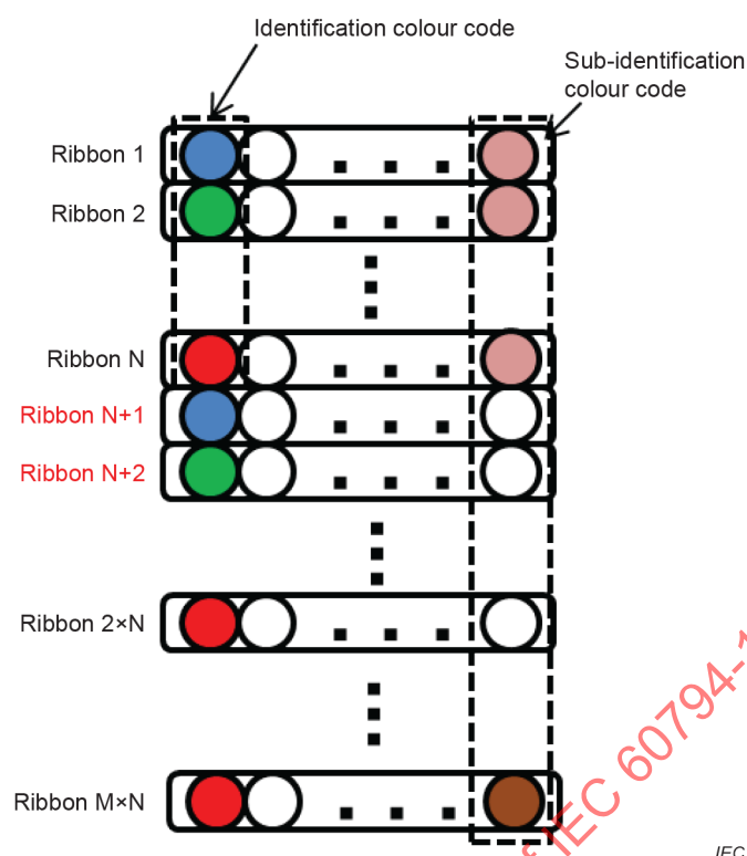
Figure A.1 – Example of identification by means of colour coding and positioning
