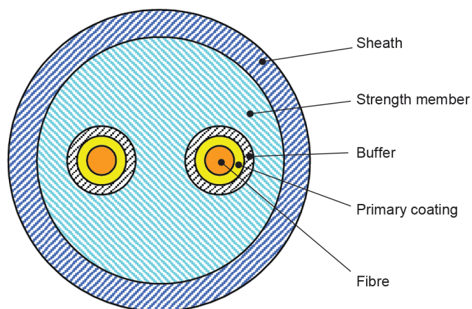
Figure A.4 – Duplex ruggedised fibre cable
