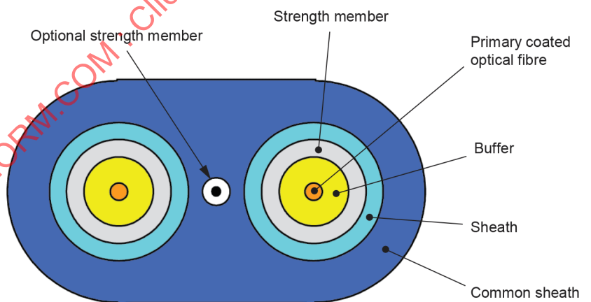
Figure A.5 – Duplex ruggedised fibre zip cord
