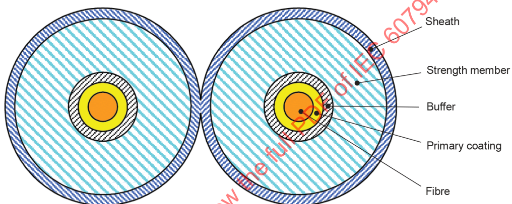
Figure A.4 – Duplex ruggedised fibre cable
