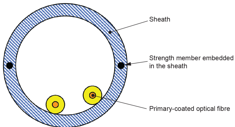
Figure A.3 – Duplex loose non-buffered fibre cable
