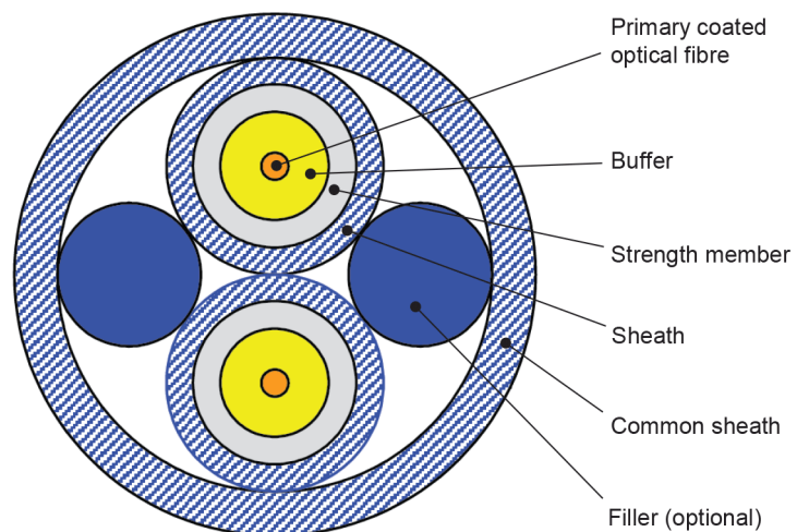
Figure A.7 – Duplex round cable
