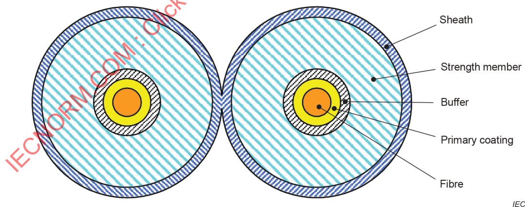
Figure A.5 – Duplex ruggedised fibre zip cord
