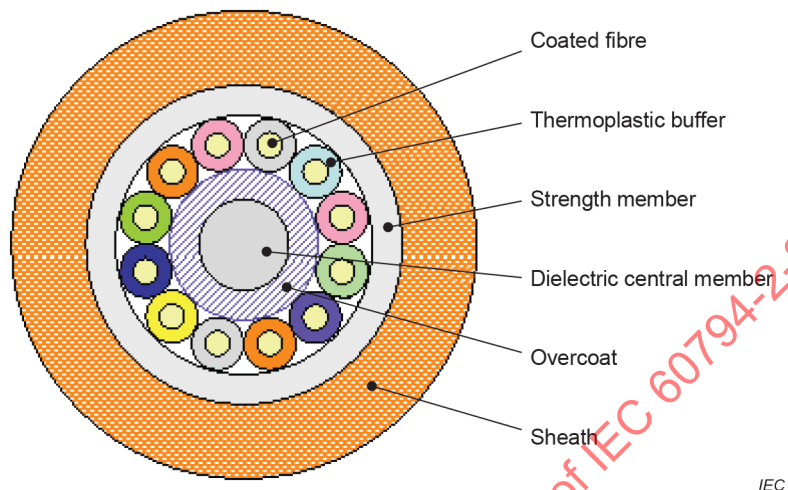
Figure A.1 – Example of cross-section of a 12-fibre cable
