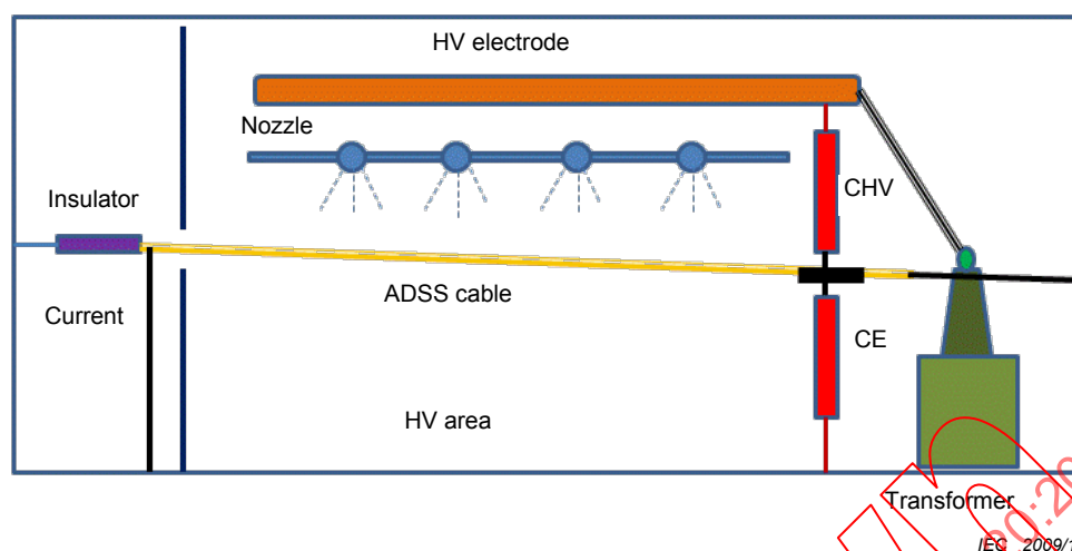
Figure C.1 – Draft of test equipment
