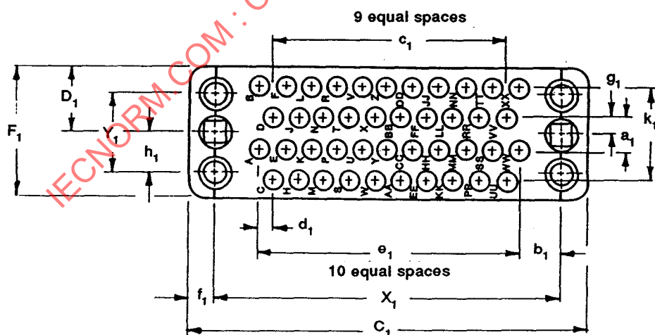
42 contact arrangement
