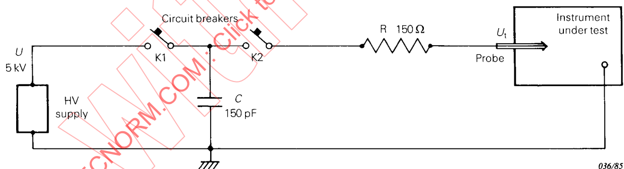
FIG. 12. — Measurement of susceptibility to electrostatic discharge.
