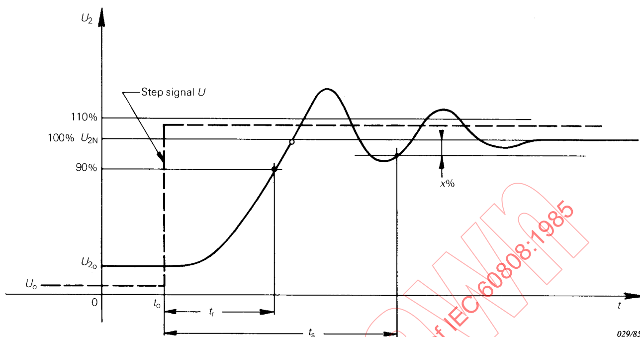
FIG. 5. — Response time.
