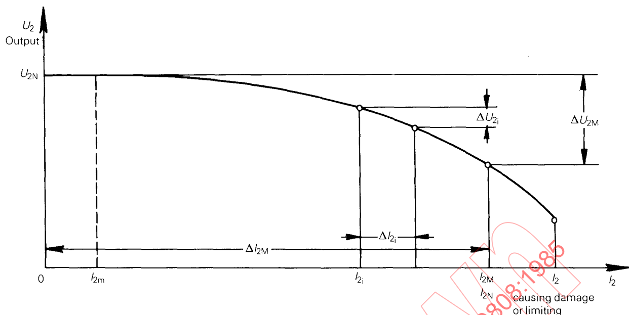
FIG. 6. — Variations as a function of load.
