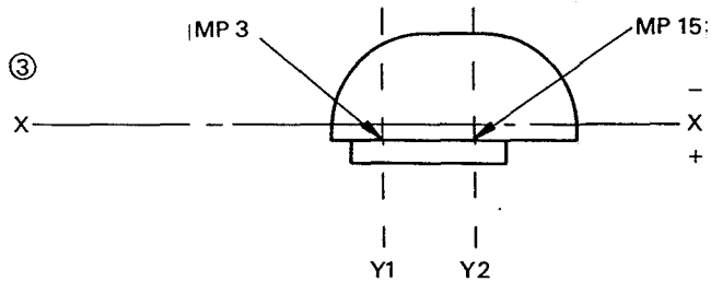
Figure D.2 – Position des points de mesure des lampes R2 Position of measuring points of R2 lamps
