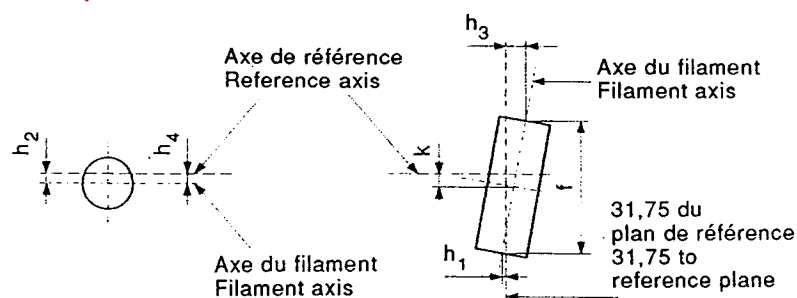
Vue A – View A
