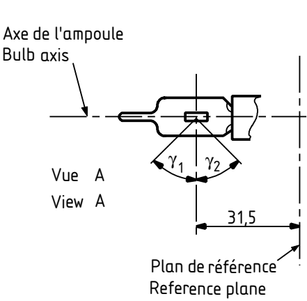
Zone exempte de distortion 5) Distortion-free area 5)
