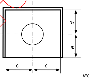
Figure J.2 – Front view of box
